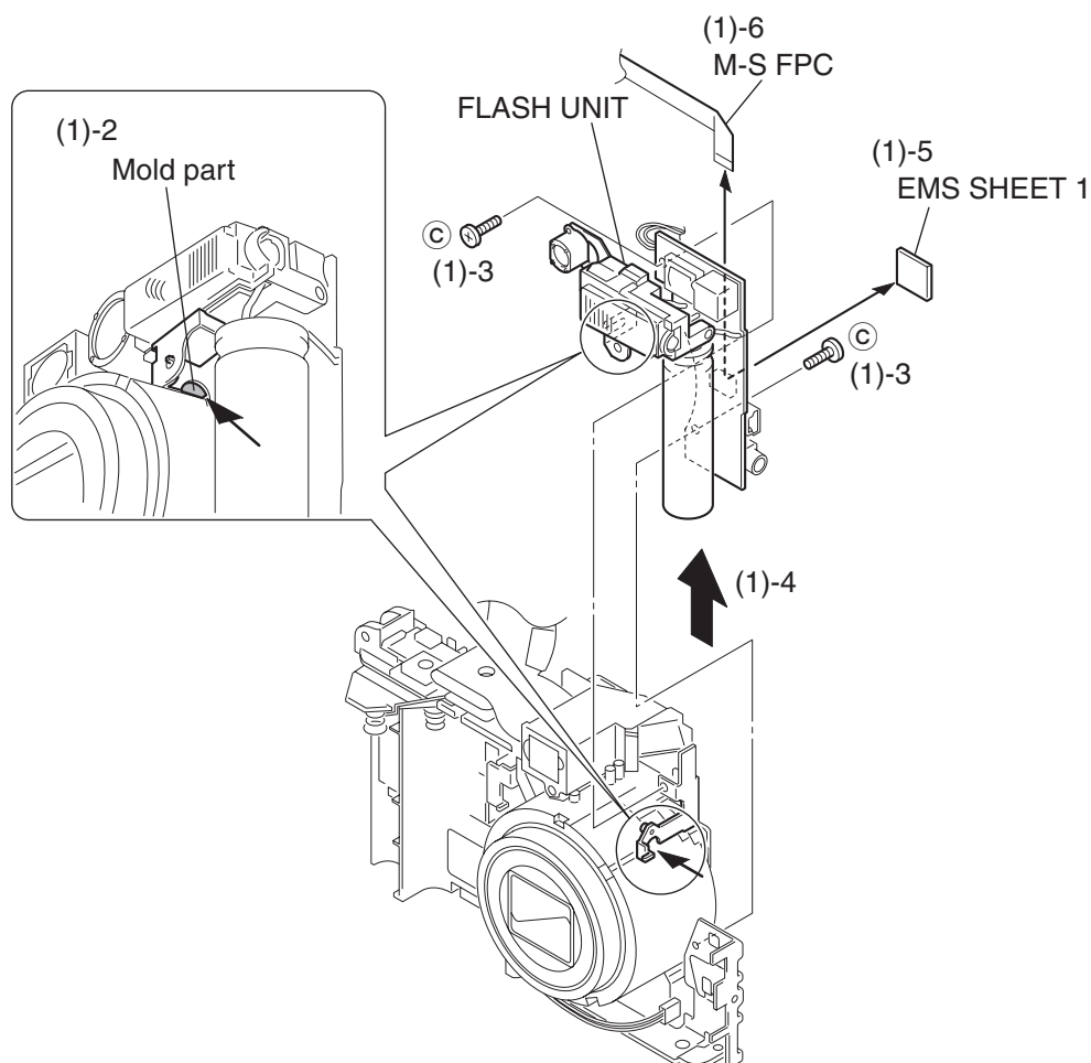
Fig. 3-10 FLASH UNIT
